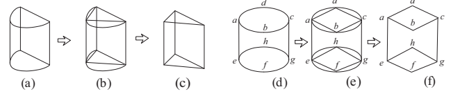
Figure 4. Examples of the transformation of line drawings, where (c) is a polyhedron and (f) is a generalized polyhedron.
