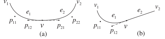
Figure 5. Illustration of curve concurrency.
