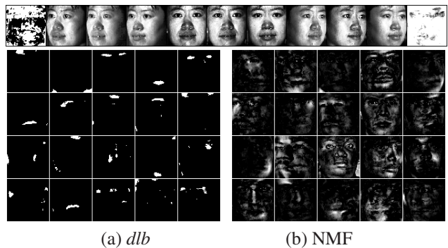
Figure 5. The first 20 bases of dlb (bottom left) and NMF (bottom right) from the CMU PIE database with multi-view faces. The top row images are: importance map image of dlb , nine sample images from the CMU PIE database, and the importance map image of NMF.
