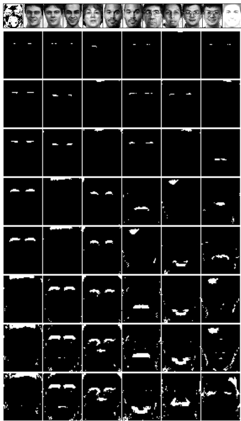
Figure 6. The first six bases (from left to right) of dlbb from the FERET database with different cardinalities (from the second row to the bottom row with the cardinality from 4 to 180); and the top row are the importance map of dlbb , ten sample images and the importance map of NMF. The results show that the bases have explicit human perceptive semantics, like eyes, mouth and nose; and when the cardinality increases, the bases can show high level structure information of a face by combining multiple components.
