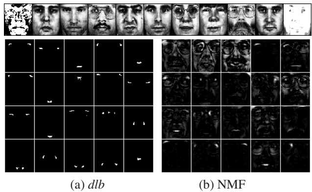
Figure 3. The first 20 bases of dlb (bottom left) and NMF (bottom right) from the XM2VTS database with well aligned frontal faces. The top row images are: importance map image of dlb , nine sample images from the XM2VTS database, and the importance map image of NMF.
