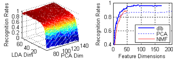
(a) U-Subspace
